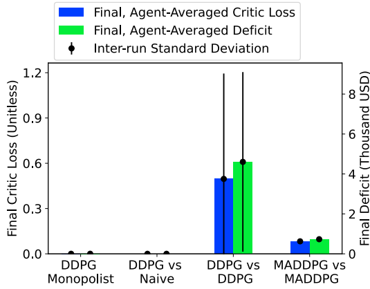
Fig. 3: Summary of the continuous environment experiment results for Case 1 (hypercompetitive, Bertrand competition). For each case, the final critic-loss and optimality-deficit are shown; uncertainty bars represent the standard deviation over all three runs. Left vertical axis corresponds to the scale of the TD-error, and the right to the deficit.
