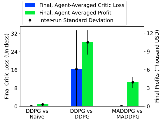
Fig. 4: Summary of the continuous environment experiment results for case 2 (competitive, Q,P-competition). For each case, the final critic-loss and profit are shown
