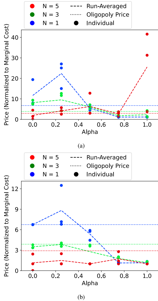
Fig. 5: Adversarial market-design: parameter-sweep summary. Plots illustrating the behavior of the final clearing price and price cap. (a) final learned price-cap. (b) clearing-price
